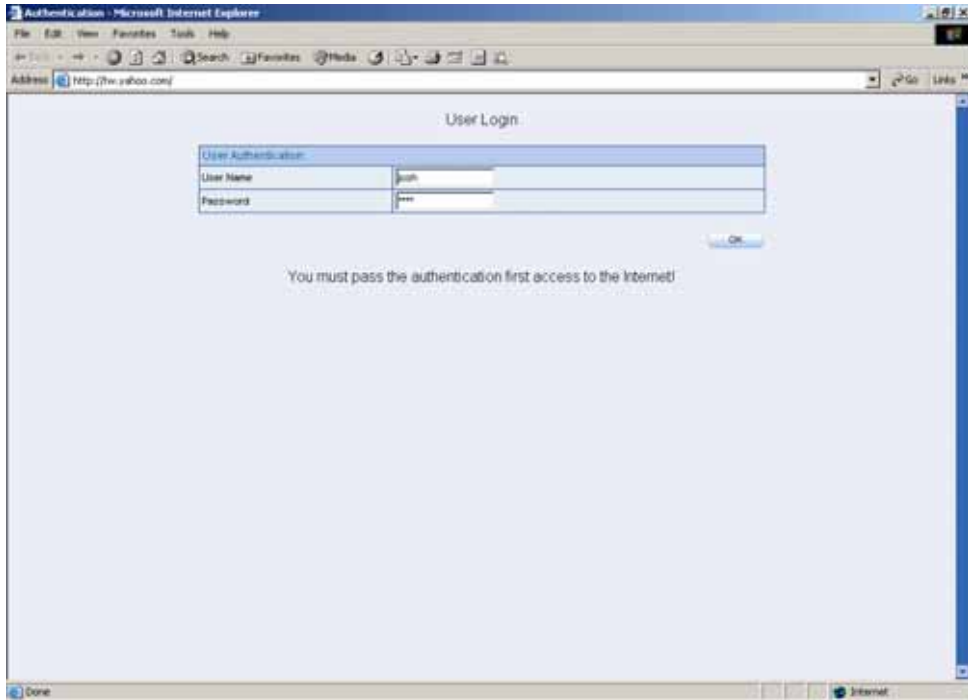
Login Authentication
